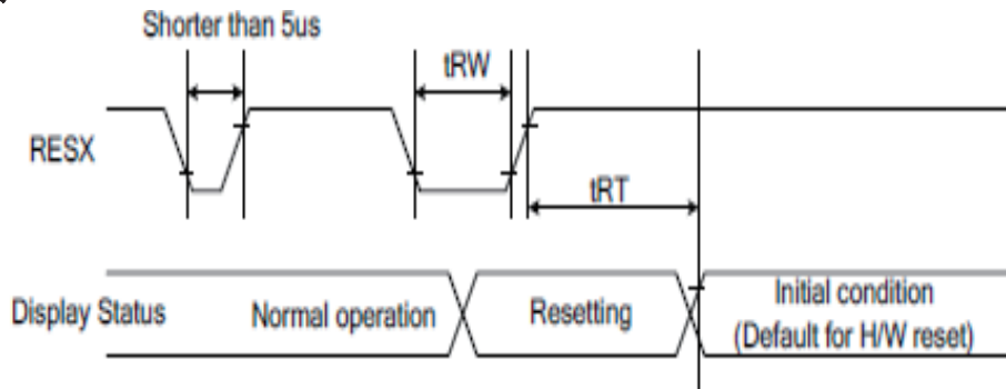
Figure 126: Reset Timing
