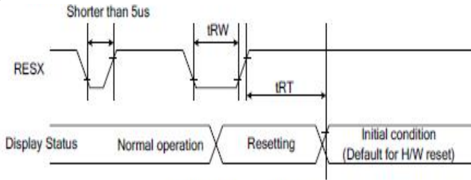
Figure 126: Reset Timing
