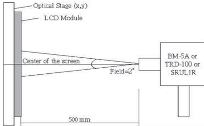
Figure 1. Optical Test Equipment Setup
