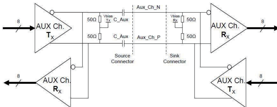
Figure 18. AUX differential pair
