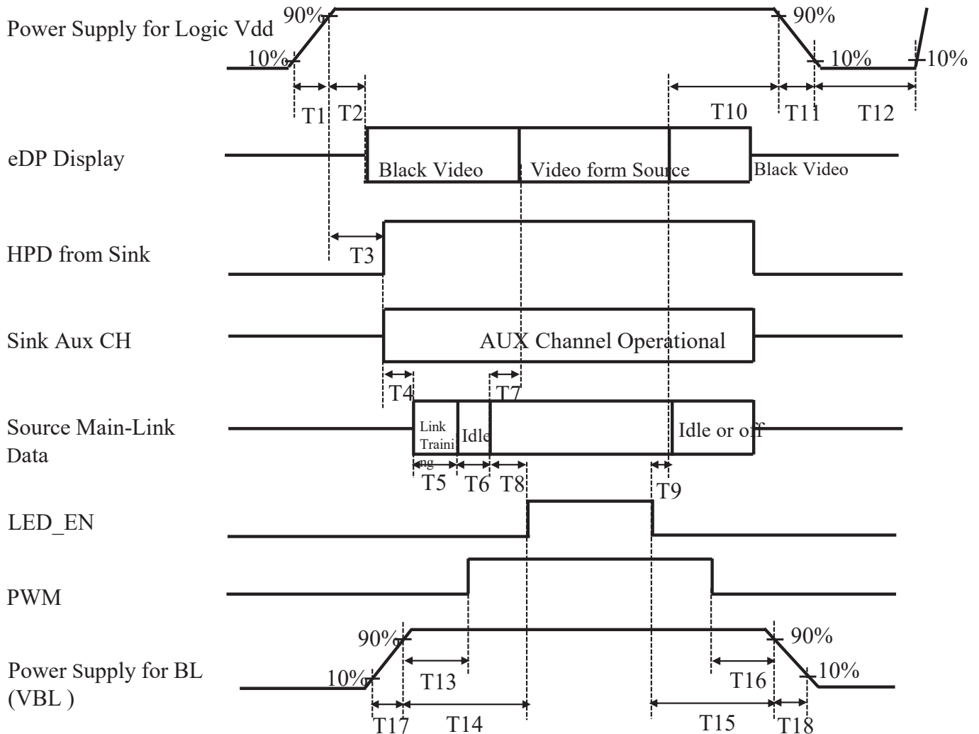
Figure 19. Power Sequence
