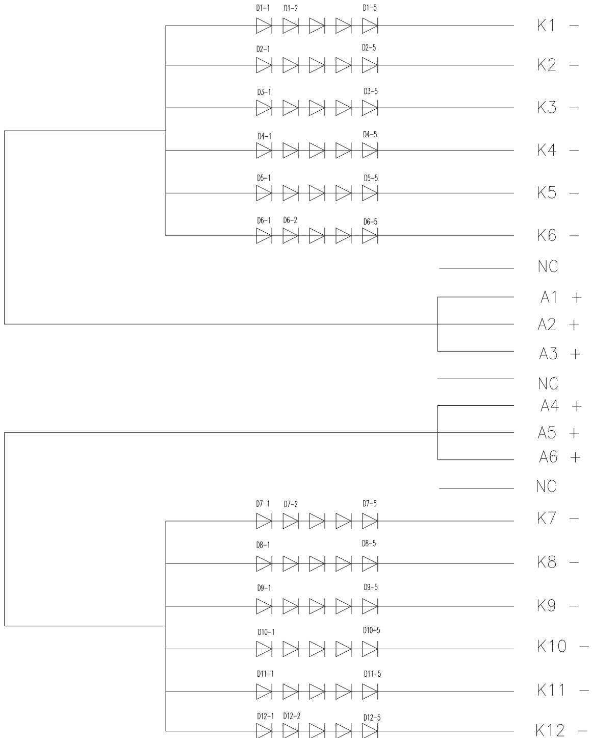
Figure 6. LED Structure
