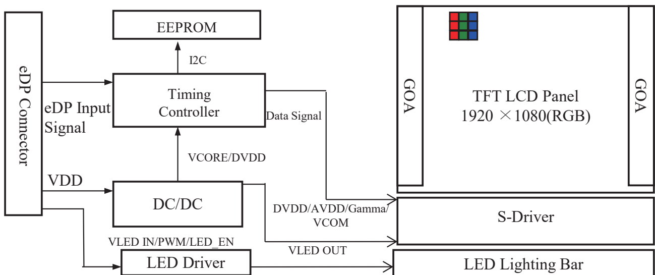
Figure 1. Drive Architecture
